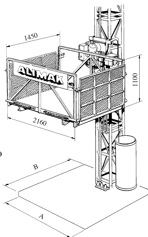
SCANDO M 1200, M 1500 & M 2000 with square mast c/c 650 x 650 mm
